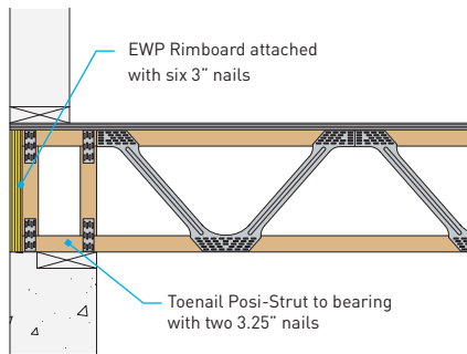
WIDE BEARING WITH RIMBOARD PS4
