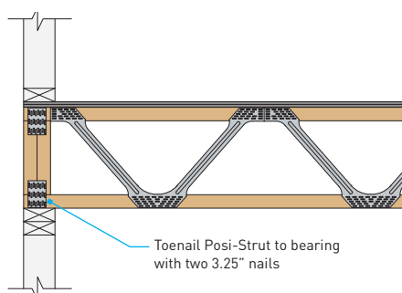
WOOD WALL BEARING WITH DOUBLE POST PS6
