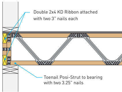
WOOD WALL BEARING WITH DOUBLE 2x4 RIBBON PS8
