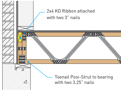
BRICK WALL WITH SINGLE 2x4 RIBBON PS1
