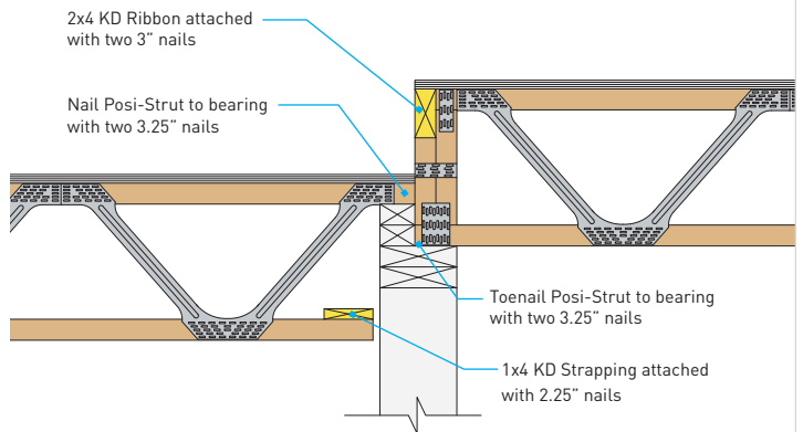
TOP CHORD / BOTTOM CHORD BEARING ASSEMBLY PS18
