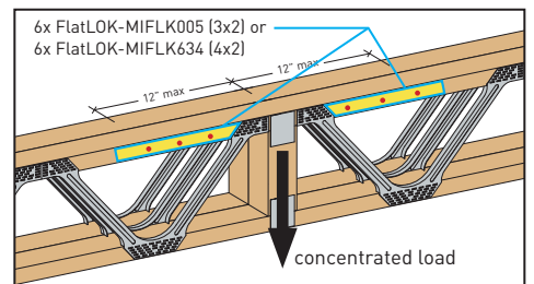
typical FlatLOK installation on Posi-Strut
