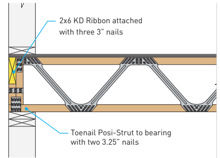
WOOD WALL BEARING WITH SINGLE 2x6 RIBBON PS9
