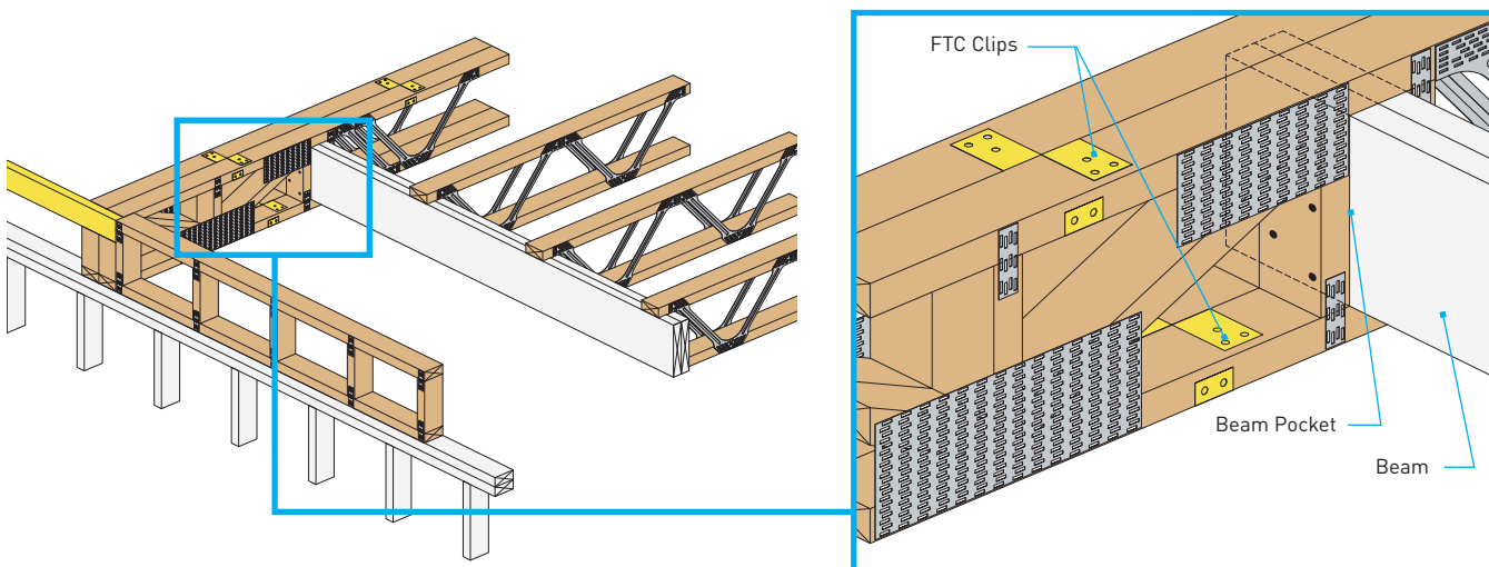
STAIRCASE ASSEMBLY WITH BEAM POCKET DETAIL PS101
