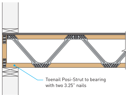
WOOD WALL BEARING WITH SINGLE POST PS5
