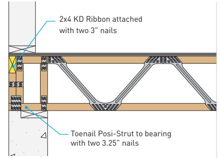
WIDE BEARING WITH SINGLE 2x4 RIBBON PS2
