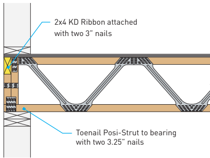
WOOD WALL BEARING WITH SINGLE 2x4 RIBBON PS7
