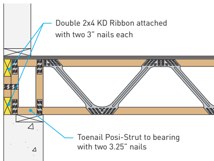
WIDE BEARING WITH DOUBLE 2x4 RIBBON PS3
