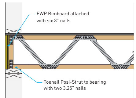
WOOD WALL BEARING WITH SINGLE POST AND RIMBOARD PS11
