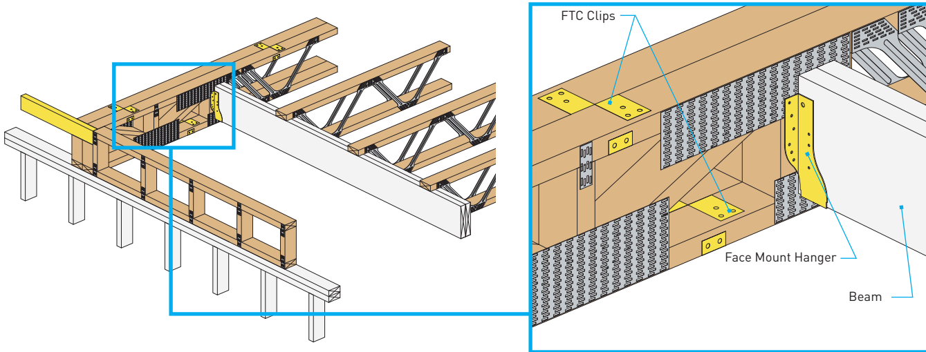
STAIRCASE ASSEMBLY WITH FACE MOUNT HANGER CONNECTION PS103
