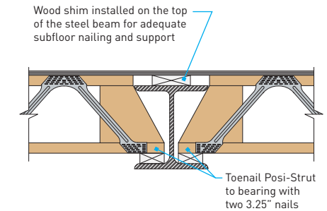
FIRE CUT DETAIL ON STEEL BEAM | PS14
